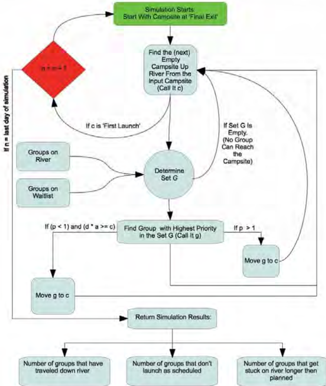
Figure 4. Visual depiction of scheduling algorithm.
